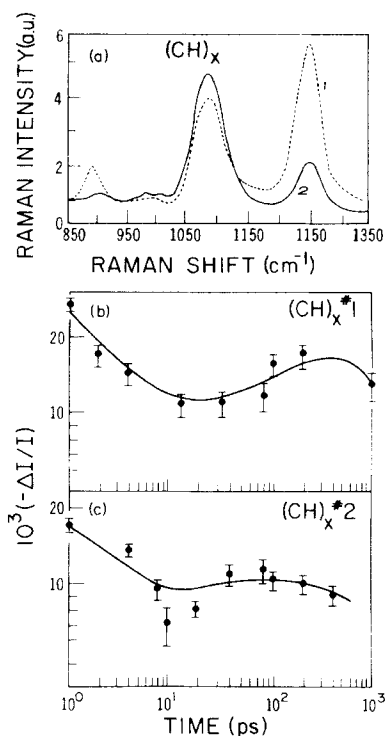
FIG. 3. (a) cw RRS spectra of partially isomerized (\text{CH})_x , No. 1 and No. 2 (see Table I) excited at 580 nm. (b),(c) TPRRS decays of (\text{CH})_x No. 1 and No. 2, respectively, excited at 580 nm and probed at 750 nm. The line through the data is a theoretical fit, see text and Table I.
