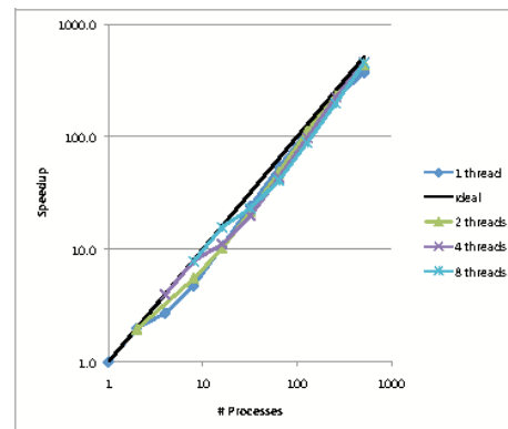
Fig. 5. Scalability of Wasatch Code.
