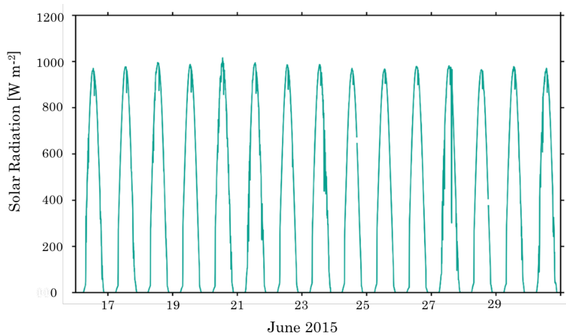
Figure 3.1 Incoming solar radiation ( \text{W m}^{-2} ) at the MTMET station in the Salt Lake Valley from 16-30 June 2015. See Figure 3.4 for the location of MTMET.
