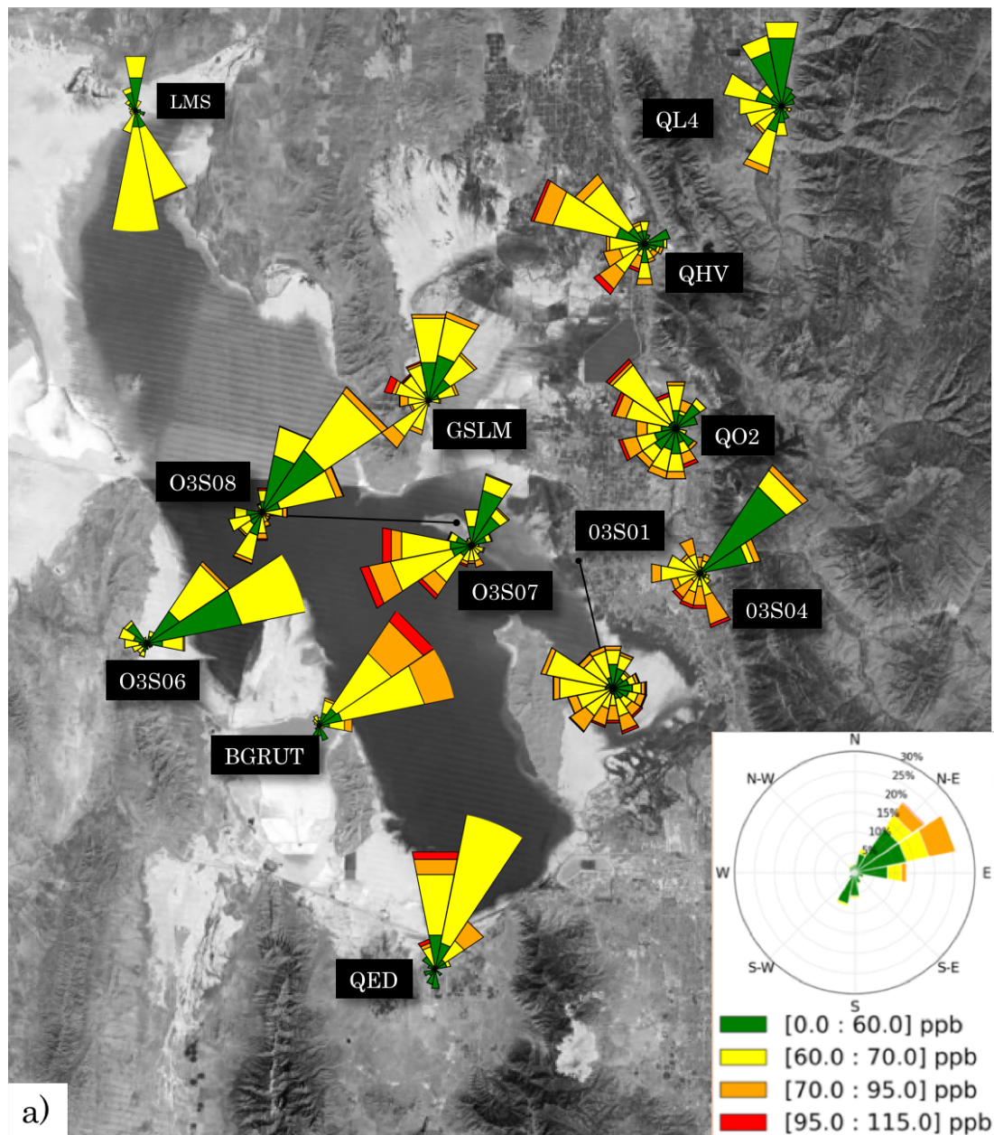
Figure 3.4. Ozone wind roses for 16-30 June 2015 during: (a,c) day (8 AM – 8 AM) and (b,d) night (8 PM – 8 AM) local time. The legend represents the length and percentages of the ozone-wind roses and the colors corresponding to ozone concentration values.
