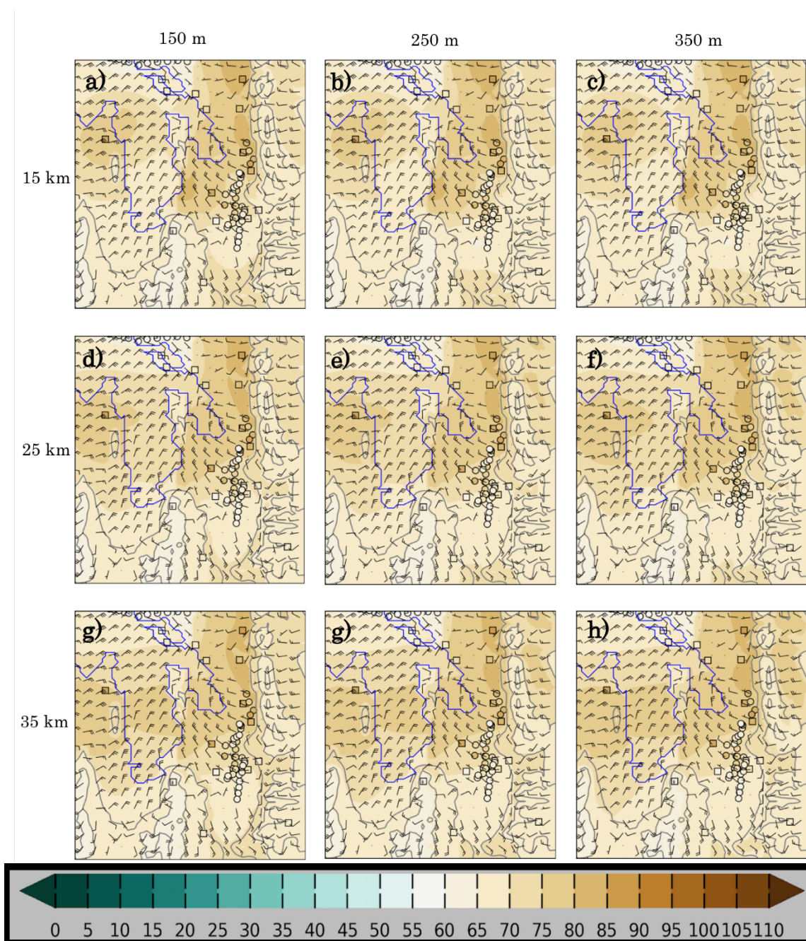
Figure 2.5. UU2DVAR sensitivity to horizontal (rows) and vertical (columns) background decorrelation length scales for 1600 MDT 18 June 2015. a)-g) show the sensitivity to the spatial ozone concentration analysis using different background decorrelation length scales. Ozone concentrations for the analyses and permanent (square) and mobile (circle) observations indicated by the colorbar (ppb). Elevation contoured in light grey at 500-m intervals beginning at 1500 m. Vector wind analyzed at every 4th gridpoint superimposed where half and full barbs denote speeds of 0.5 and 1.0- \text{m s}^{-1} .
