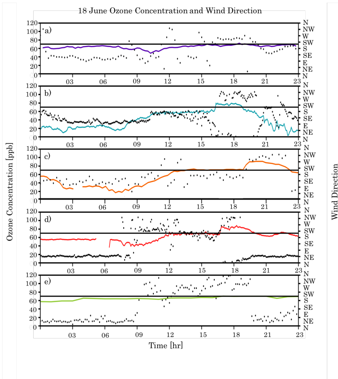
Figure 3.6. Time series of ozone (ppb) and wind direction (circles) at: a) Farnsworth Peak (FWP), b) Neil Armstrong Academy (NAA), c) Hawthorne (DAQ), d) Mountain Meteorology Lab (MTMET), and e) Snowbird (S2OZN).
