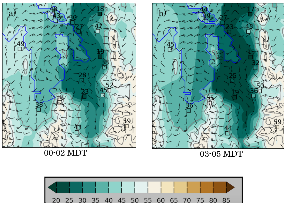
Figure 3.10. Composite ozone concentration analyses averaged over 3-hr blocks during the period 16-30 June 2015 shaded according to the colorbar. Composite vector wind analyses at every 4th gridpoint superimposed where half and full barbs denote speeds of 0.5 and 1.0- \text{m s}^{-1} . Averaged ozone concentrations during those periods are indicated at fixed sites (squares). Elevation contoured in light grey at 500-m intervals beginning at 1500 m. (a-h) Shows 3-hr average ozone concentration analysis (in ppb).
