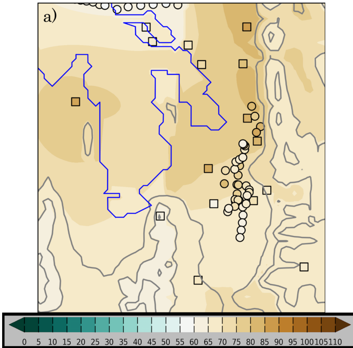
Figure 2.4. UU2DVAR ozone concentration analysis (in ppb with shading according to the colorbar) for 1600 MDT 18 June 2015. Observations from fixed sites are denoted by squares while mobile observations used in the analysis are denoted by circles. Elevation is contoured in light grey at 500-m intervals beginning at 1500 m. a) UU2DVAR ozone concentration (in ppb) analysis with fixed site observations and mobile observations. b) UU2DVAR ozone concentration (in ppb) analysis using only fixed site observations. c) Ozone concentration difference (in ppb) between the analysis using all available observations and the analysis without mobile observations.
