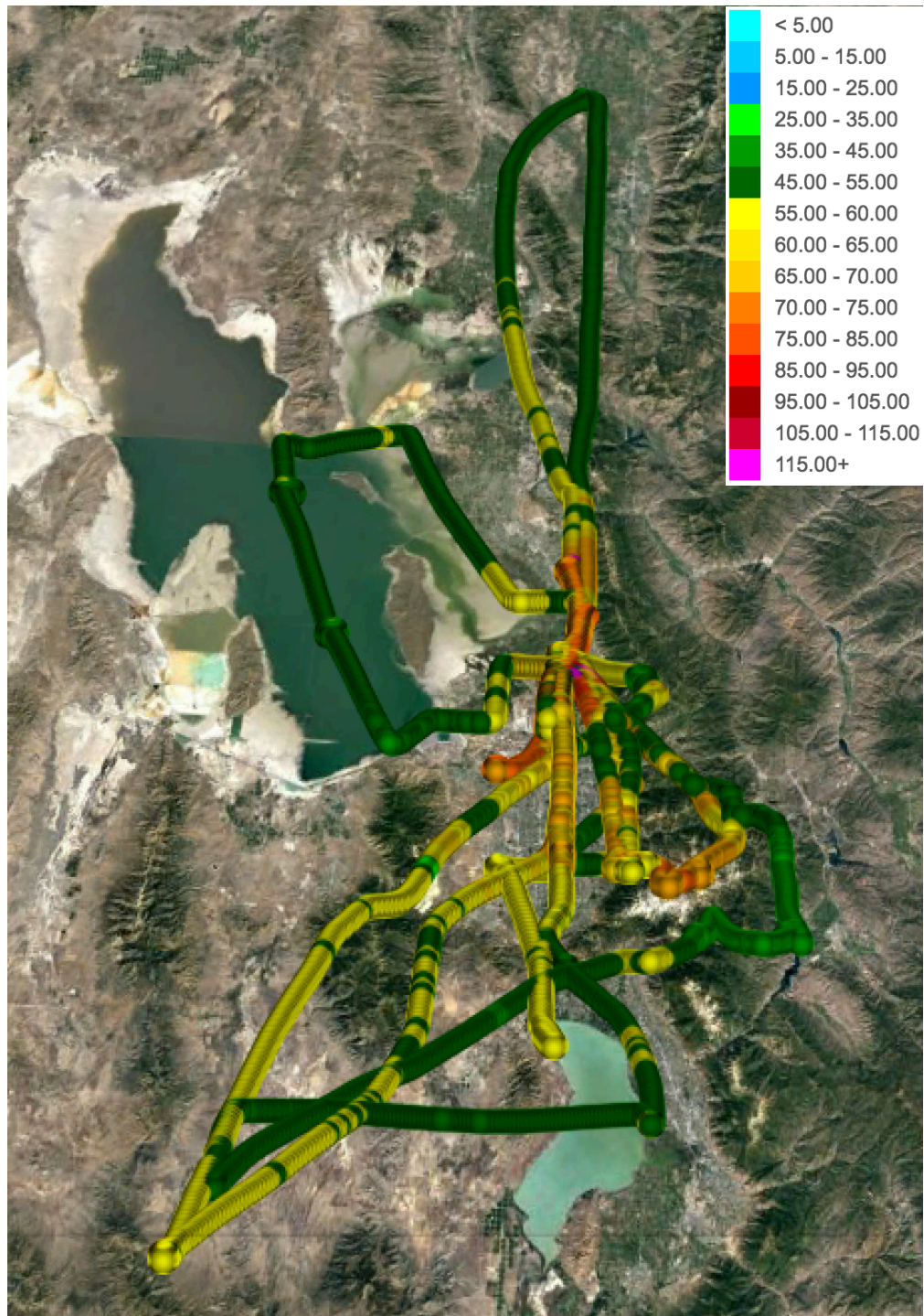
Figure 2.2. Flight paths available from the KSL News helicopter during the 16-30 June 2015 period. Ozone concentrations (ppb) are denoted according to the scale in the upper right.
