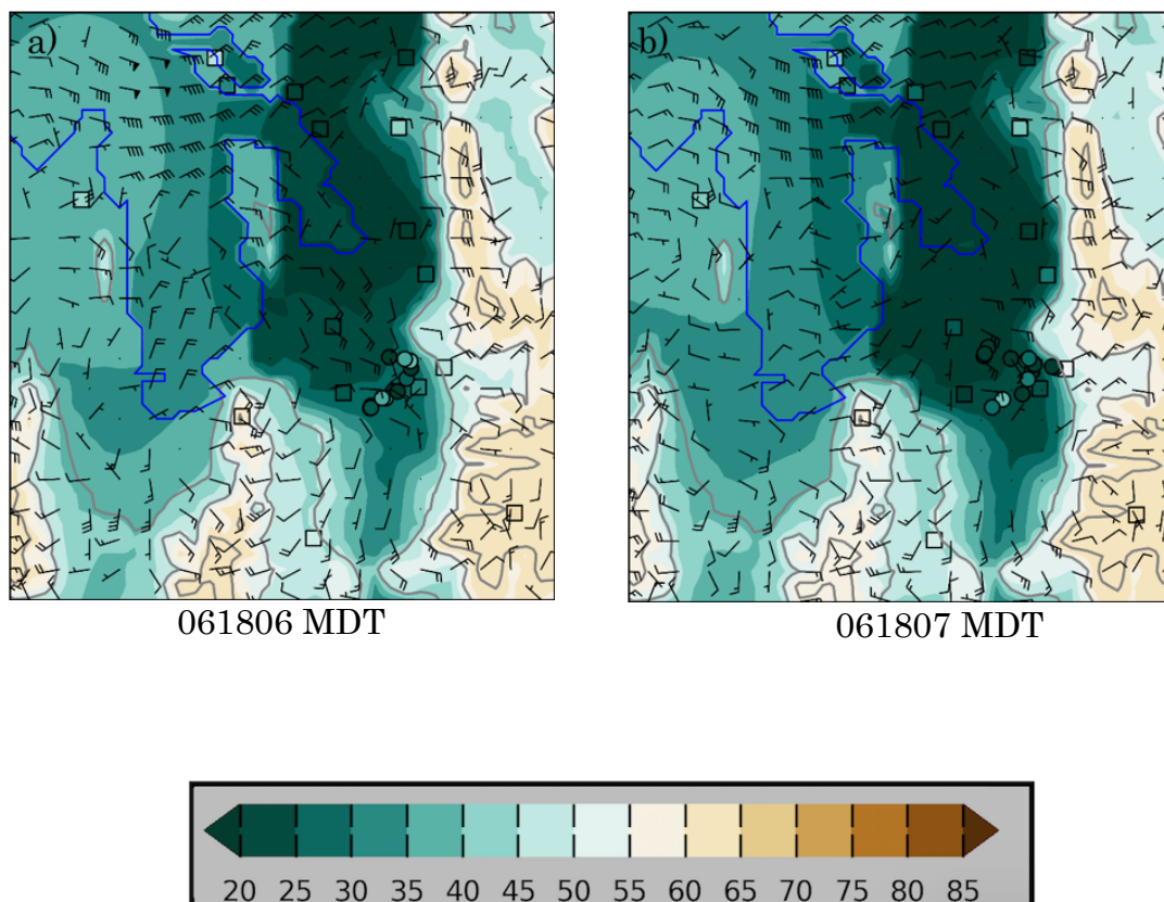
Figure 3.7. Ozone concentration analyses shaded according to the colorbar during 18 June 2015 at hourly intervals from 0600 – 2300 MDT. Vector wind analyses at every 4th gridpoint superimposed where half and full barbs denote speeds of 0.5 and 1.0- \text{m s}^{-1} . Observations of ozone concentrations at fixed sites (squares) and from mobile observations (circles) are shown using the same colorbar. Elevation contoured in light grey at 500-m intervals beginning at 1500 m. (a-r) Shows hourly analysis of ozone concentration (in ppb).
