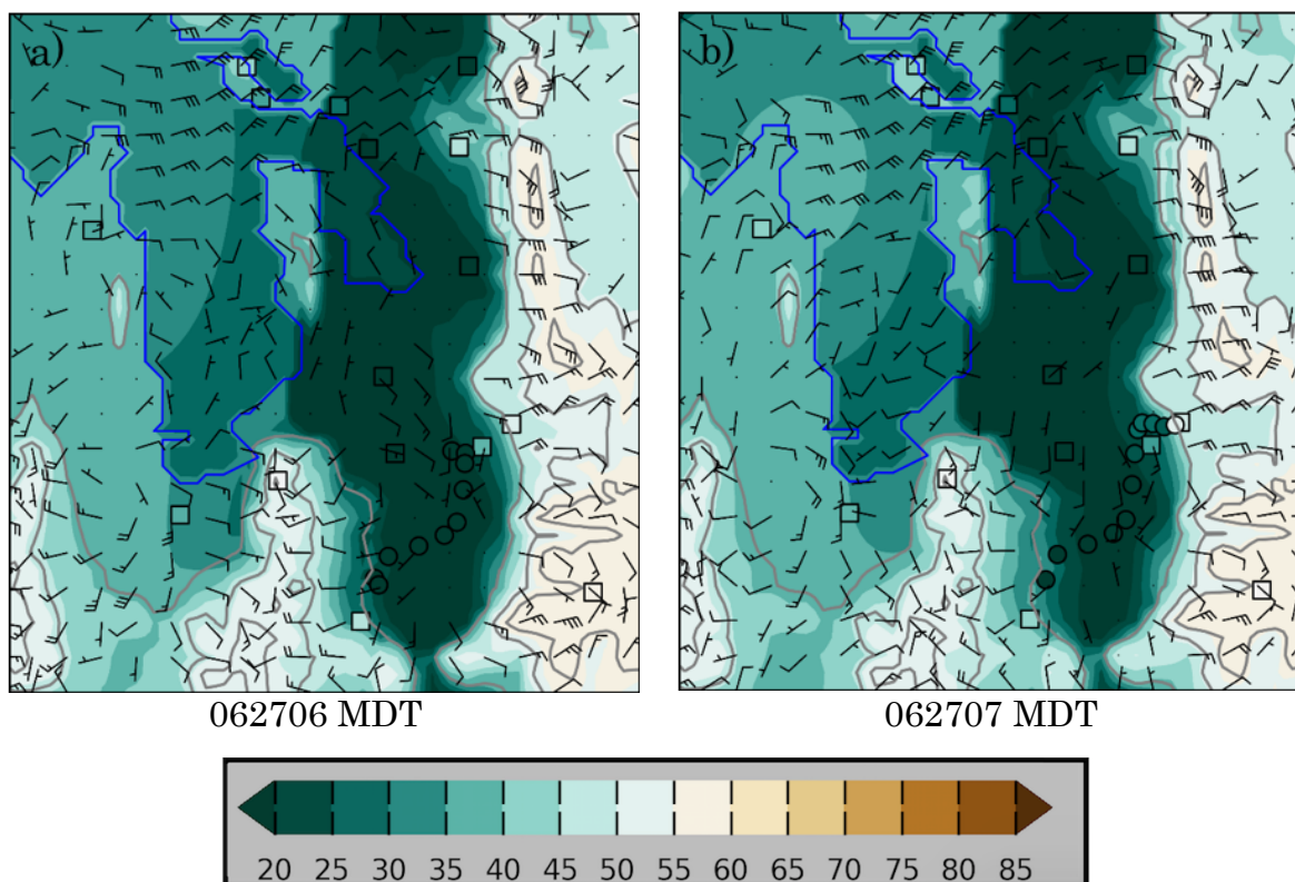
Figure 3.9. Ozone concentration analyses shaded according to the colorbar during 27 June 2015 at hourly intervals from 0600 – 2300 MDT. Vector wind analyses at every 4th gridpoint superimposed where half and full barbs denote speeds of 0.5 and 1.0- \text{m s}^{-1} . Observations of ozone concentrations at fixed sites (squares) and from mobile observations (circles) are shown using the same colorbar. Elevation contoured in light grey at 500-m intervals beginning at 1500 m. (a-r) Shows hourly analysis of ozone concentration (in ppb)
