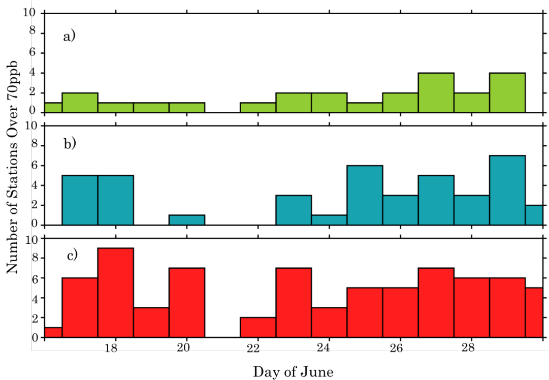
Figure 3.2. Number of stations in the a) rural, b) lakeshore, and c) urban categories from 16-30 June 2015 that exceed 70 ppb during an 8-hr period.
