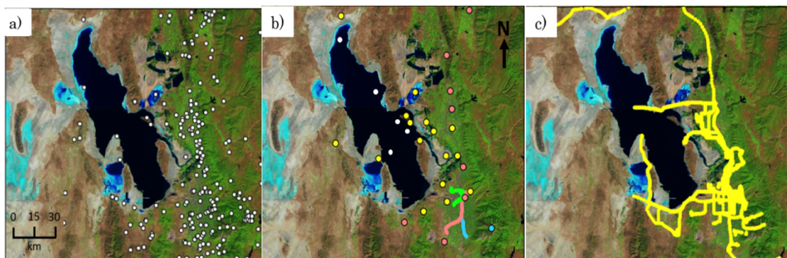
Figure 2.1. Location of selected instrumentation during the GSLSO 3 S. a) meteorological monitoring locations. b) ozone monitoring at permanent DAQ (red circles) and United States Forest Service (blue circle) sites, season-long sites (yellow circles), bogus ozone sites assumed from lakeshore locations over GSL (white circles) as well as routes of the light-rail car on Red, Green, and Blue lines in the Salt Lake Valley. c) cumulative ozone monitoring routes of vehicles (yellow).
