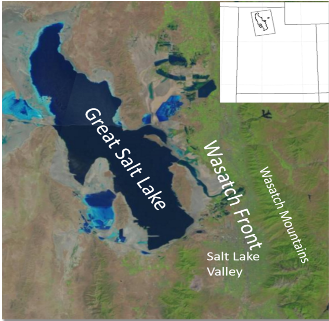
Figure 1.1. Region of interest for this study and areal extent of the Great Salt Lake during summer 2015.
