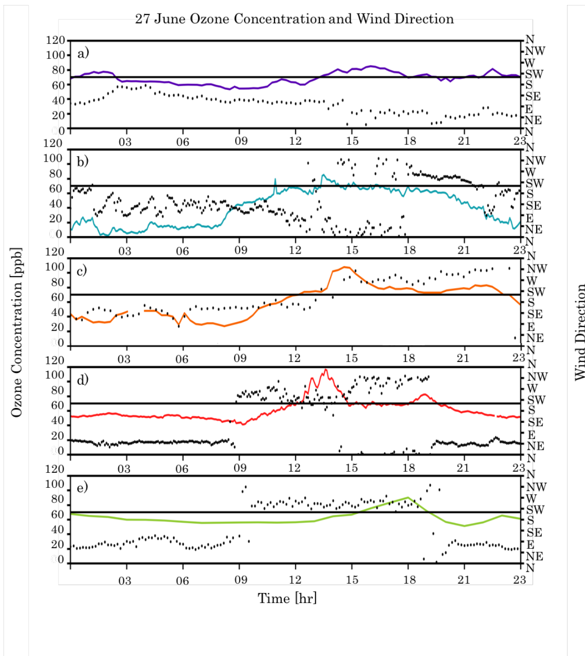
Figure 3.8. Time series of ozone (ppb) and wind direction at: a) Farnsworth Peak (FWP), b) Neil Armstrong Academy (NAA), c) Hawthorne (DAQ), d) Mountain Meteorology Lab (MTMET), and e) Snowbird (S2OZN).
