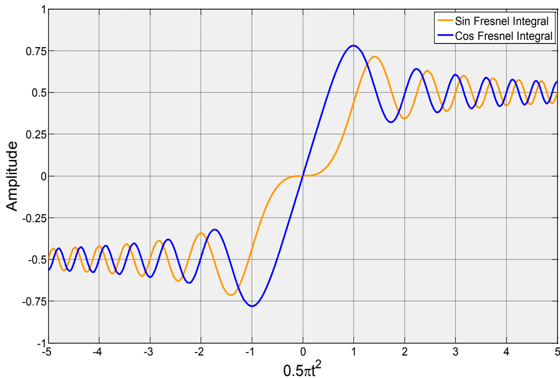
Figure 16. Plot of the sine and cosine components of the Fresnel integral C[v] = \int_0^v \text{Cos} \left[ \frac{\pi t^2}{2} \right] dt and S[v] = \int_0^v \text{Sin} \left[ \frac{\pi t^2}{2} \right] dt . Both of these two integrals go to \pm \frac{1}{2} as t \rightarrow \pm \infty .
