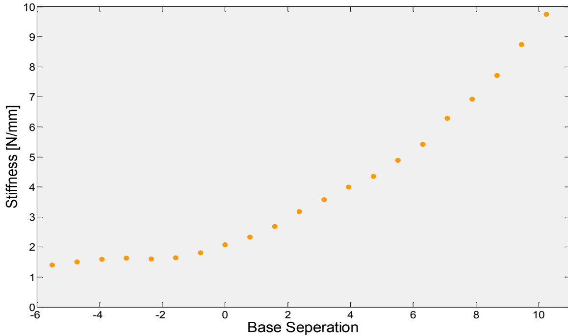
Figure 26. The linear stiffness coefficient as a function of base displacement d .
