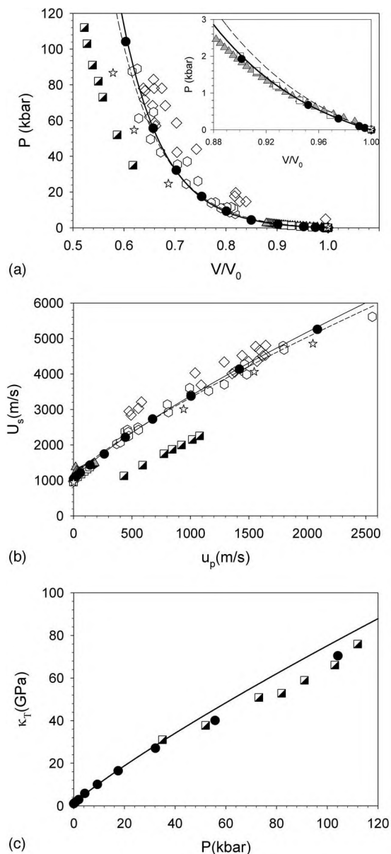
FIG. 2. (a) Comparison of experimental and simulation pressure vs compression data for Sylgard®/PDMS. Symbols represent data points from Dattelbaum et al. (Ref. 1) (diamonds), Marsh (Ref. 37) (hexagons), Sachdev et al. (Ref. 35) (triangles), Stevens et al. (Ref. 38) dilatometry (squares, empty) and Brillouin (squares, half-filled) experiments, and Dattelbaum et al. 470 g/mol (pure) PDMS (Ref. 36) (stars) and simulation (circles). The lines represent the fitted Tait EOS for both fitted (solid) and universal (dashed) values of C to the simulation data. The inset expands the low-pressure region of the data. (b) Comparison of the experimental and simulation U_s - u_p data for Sylgard®/PDMS. All symbols and lines are as in (a). (c) Comparison of the experimental and simulation bulk modulus for Sylgard®/PDMS. All symbols and lines are as in (a).
