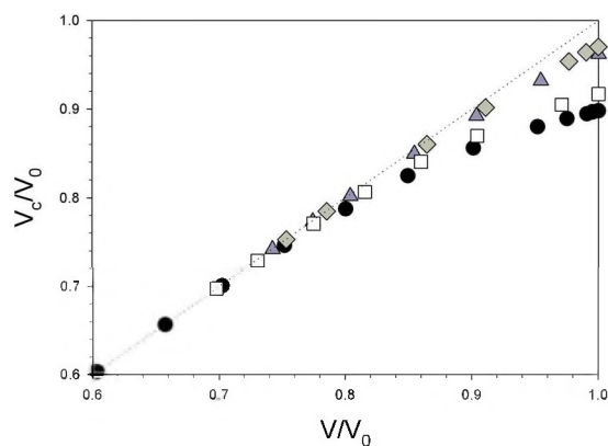
FIG. 10. (Color online) The core volume ( V - V_f ) normalized by the zero-pressure volume V_0 as a function of compression ratio for PDMS (circles), PBD (squares), np-Estane (triangles), and model Estane ® (diamonds). The dashed line represents the asymptotic limit wherein compression has removed all the free volume from the system and the core volume ratio is equivalent to the overall compression ratio.
