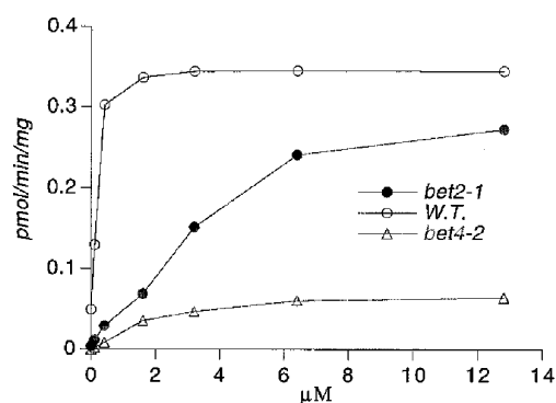
FIG. 9. Saturation curves for [ ^3 H]GGPP using wild type ( W.T. ) (open circle), bet2-1 (solid circle), and bet4-2 (open triangle) mutant extracts. Assays were performed at 30 °C for 30 min with 25 \mu g of yeast extract and the indicated concentration of [ ^3 H]GGPP. Each value is an average of duplicate determinations.
