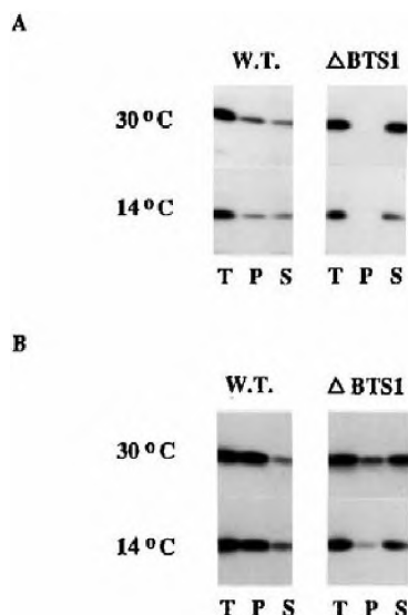
FIG. 7. The membrane attachment of Ypt1p and Sec4p is defective in \Delta BTS1 cells. Cells were grown at 30 °C to exponential phase. 1 aliquot of cells was removed, pelleted, converted to spheroplasts, and lysed. The remaining cells were shifted to 14 °C and grown for 12 h before they were harvested and lysed. Lysates ( T ) were centrifuged at 100,000 \times g to obtain pellet ( P ) and supernatant ( S ) fractions. Samples were electrophoresed on a 12.5% SDS-polyacrylamide gel and subjected to Western blot analysis using anti-Ypt1p (A) or anti-Sec4p (B) antibodies. W.T. , wild type.
