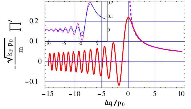
FIG. 2 (color online). Derivative \Pi' of the polarization operator is plotted from Eq. (4) versus dimensionless deviation \delta q/p_0 = (q - 2k_F)/p_0 from the Kohn anomaly. Dashed line shows \Pi' in a zero magnetic field. Inset: \Pi' is plotted from Eq. (9) at temperatures 2\pi T = \epsilon_0 (1) and 2\pi T = 1.5\epsilon_0 (2).
