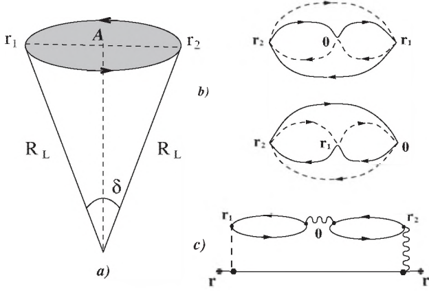
FIG. 1. (a) Origin of the “magnetic” term in the argument Eq. (2): two arcs, corresponding to the opposite directions of propagation, define a finite area \mathcal{A} . (b) Three-scattering processes responsible for magnetic field dependence of the relaxation rate are illustrated schematically. (c) One of three RPA-type diagrams describing the B -dependent correction to the density of states in the ballistic regime: scattering by the impurity occurs at point \mathbf{r}_1 ; two electron-electron scattering acts occur at points \{\mathbf{r}_1, \mathbf{r}_2\} .
