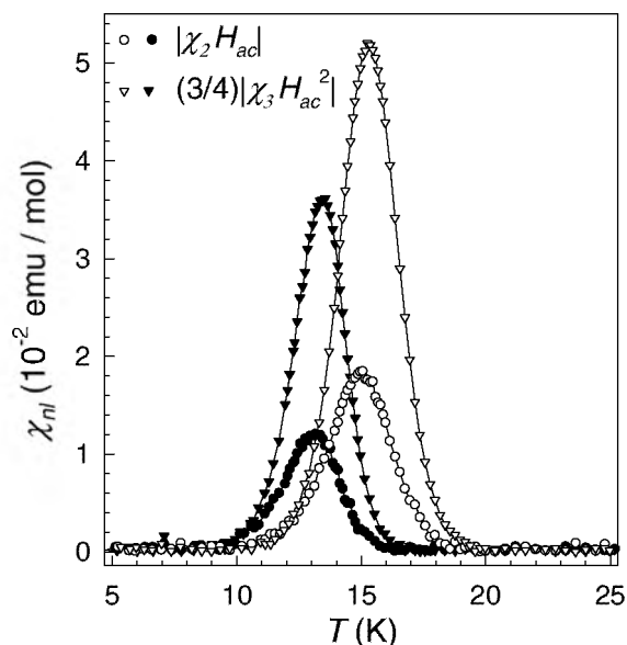
FIG. 4. Nonlinear ac susceptibility ( x \approx 0.3 sample) at H_{ac} = 15 Oe, f = 110 Hz, for the ground and photoexcited states (solid and open symbols, respectively).
