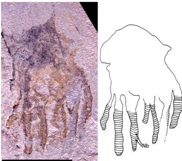
Figure 11. Photograph and interpretive drawing of Middle Cambrian cnidarian jellyfish in lateral view possibly referable to the class Cubozoa. Specimen UU07021.02, scale bar equals 5 mm. Structures marked Nb in drawing are interpreted as nematocyst batteries. doi:10.1371/journal.pone.0001121.g011
