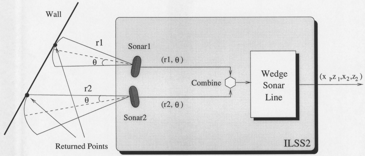
Figure 2: Two Instrumented Logical Sensors for determining wall position.
