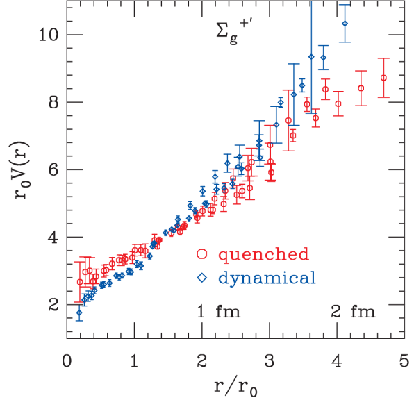
Figure 2. The excited \Sigma_g^{+'} potential for quenched (octagons) and 2+1 flavor (diamonds) QCD, in units of r_0 . The lattice spacing was matched using r_0 .
