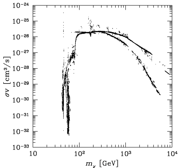
Fig. 3.— Scatter plot of neutralino annihilation cross section versus neutralino mass for supersymmetric models that satisfy accelerator and WMAP constraints. A typical cross-section (assumed in our estimates) is \sigma v \approx 2 \times 10^{-26} \text{cm}^3 \text{s}^{-1} .
