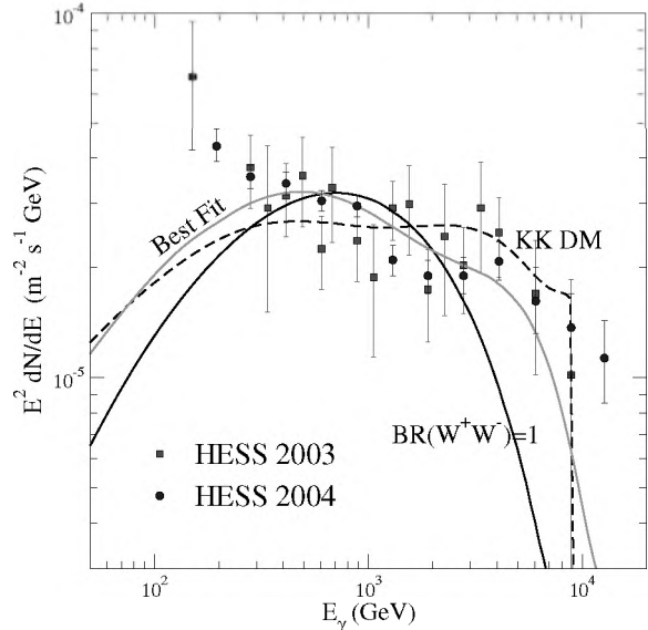
Fig. 4.— The HESS 2003 (grey squares) and HESS 2004 (filled circles) data on the flux of GR from the GC, and the best fit to those data with a KK B^{(1)} pair-annihilating lightest KK particle (dashed line), with a WIMP annihilating into a W^+W^- pair (black solid line), and with the best WIMP spectral function fit (light grey line).
