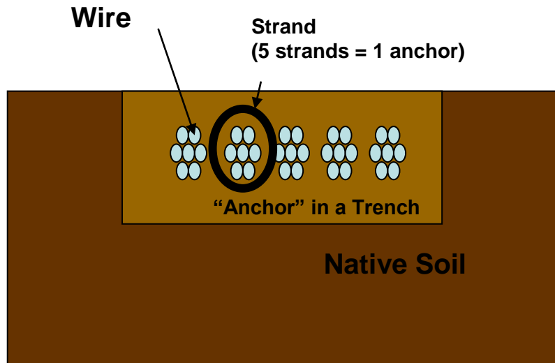
Fig. 9. Cross Section of Simulated Anchor for this Test. Another identical anchor in another trench a few feet away was used as the 'ground' reference. © 2009 IEEE. Reprinted, with permission, from 39.
