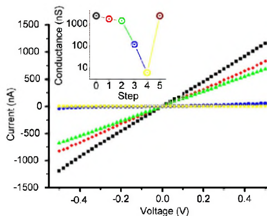
FIG. 3. (Color online) Conductance transition corresponds to the bending process at low temperature (30 K). Conductance dropped when bending the nanowire step-by-step (from the first step to the fourth step) and reverted to the initial state when the middle tip was retracted to release the nanowire to its original shape (fifth step).
