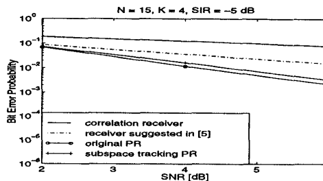
Figure 2: Bit error probability for different receivers.
