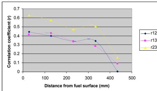
Figure 7. Correlation trends with height for JP8
