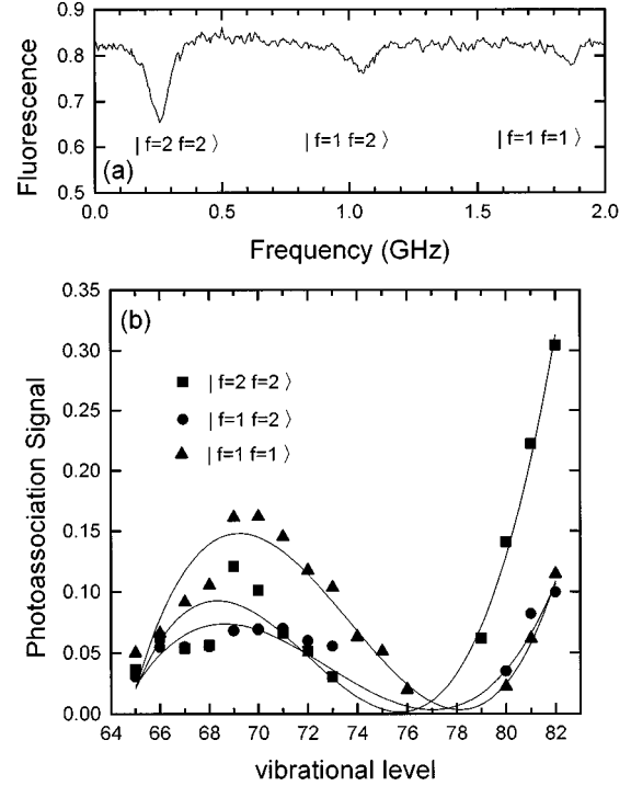
FIG. 2. (a) Spectrum of the v=81, N=1 level of the A^1\Sigma_u^+ state of {}^7\text{Li}_2 . Three features, separated by the atomic ground-state hyperfine splitting, are observed corresponding to collisions with both atoms having f=2 , one atom with f=1 and the other with f=2 , and both atoms having f=1 . The fluorescence is given in arbitrary units. (b) Photoassociation signals for each hyperfine feature of each vibrational level of the A^1\Sigma_u^+ state of {}^7\text{Li}_2 . The lines are a polynomial fit to the data to help identify the node for each hyperfine series. The resulting minimum in the photoassociation signal occurs at a different location for the different collision channels.
