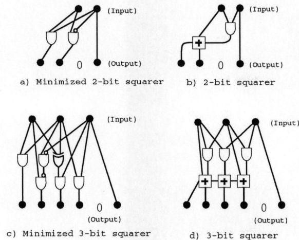
Figure 3: Primitive squarers
