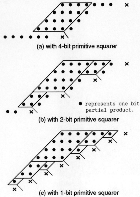
Figure 2: 8-bit squarers
