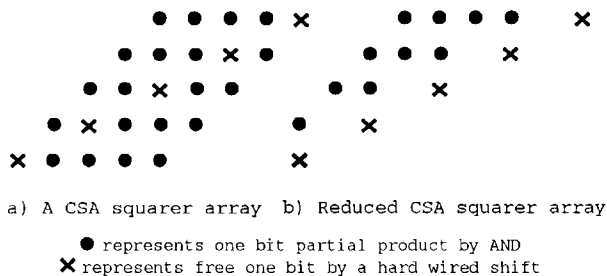
Figure 1: CSA squarers
