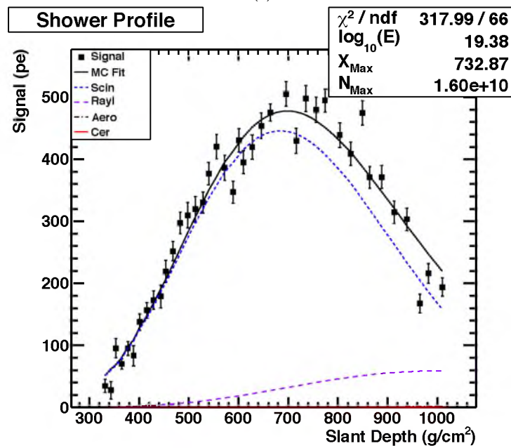
Figure A.10. Continuation of the ninth highest energy event in the Middle Drum hybrid data set: it was recorded on 11/16/2009 at 9:10:14 UTC. Shown are (c) the timing vs. angle plot for the geometry reconstruction, and (d) the plot of the shower profile (signal as a function of atmospheric depth).
