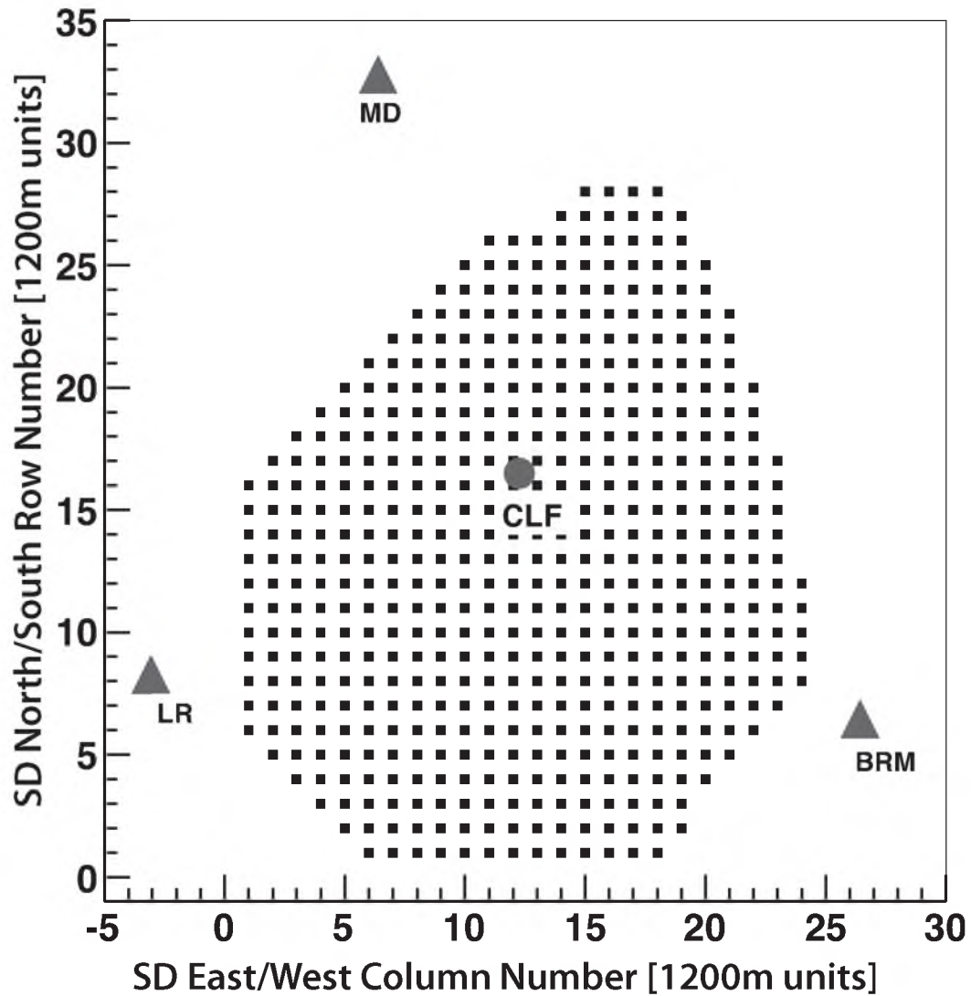
Figure 3.1. The layout of the Telescope Array experiment: the different components of the experiment are indicated on this map. The filled black squares indicate the locations of the scintillation counters that comprise the Surface Detector (SD). The triangles mark the three fluorescence detector sites at the periphery of the SD array. The Central Laser Facility, shown by the circle, is placed equidistant from the three fluorescence detection sites to provide atmospheric monitoring and cross-calibration.
