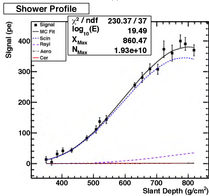
Figure A.6. Continuation of the fifth highest energy event in the Middle Drum hybrid data set: it was recorded on 9/28/2008 at 5:43:03 UTC. Shown are (c) the timing vs. angle plot for the geometry reconstruction, and (d) the plot of the shower profile (signal as a function of atmospheric depth).
