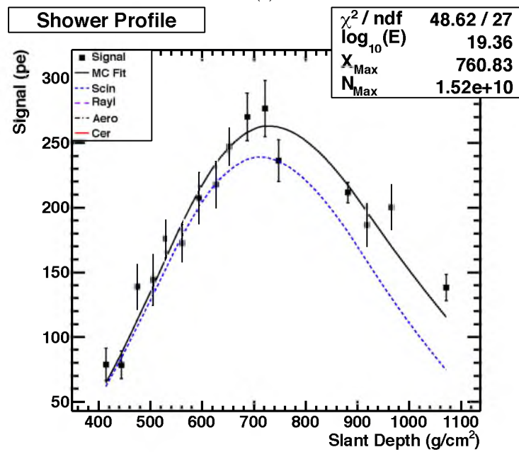
Figure A.11. Continuation of the tenth highest energy event in the Middle Drum hybrid data set: it was recorded on 5/05/2011 at 5:52:14 UTC. Shown are (c) the timing vs. angle plot for the geometry reconstruction, and (d) the plot of the shower profile (signal as a function of atmospheric depth).
