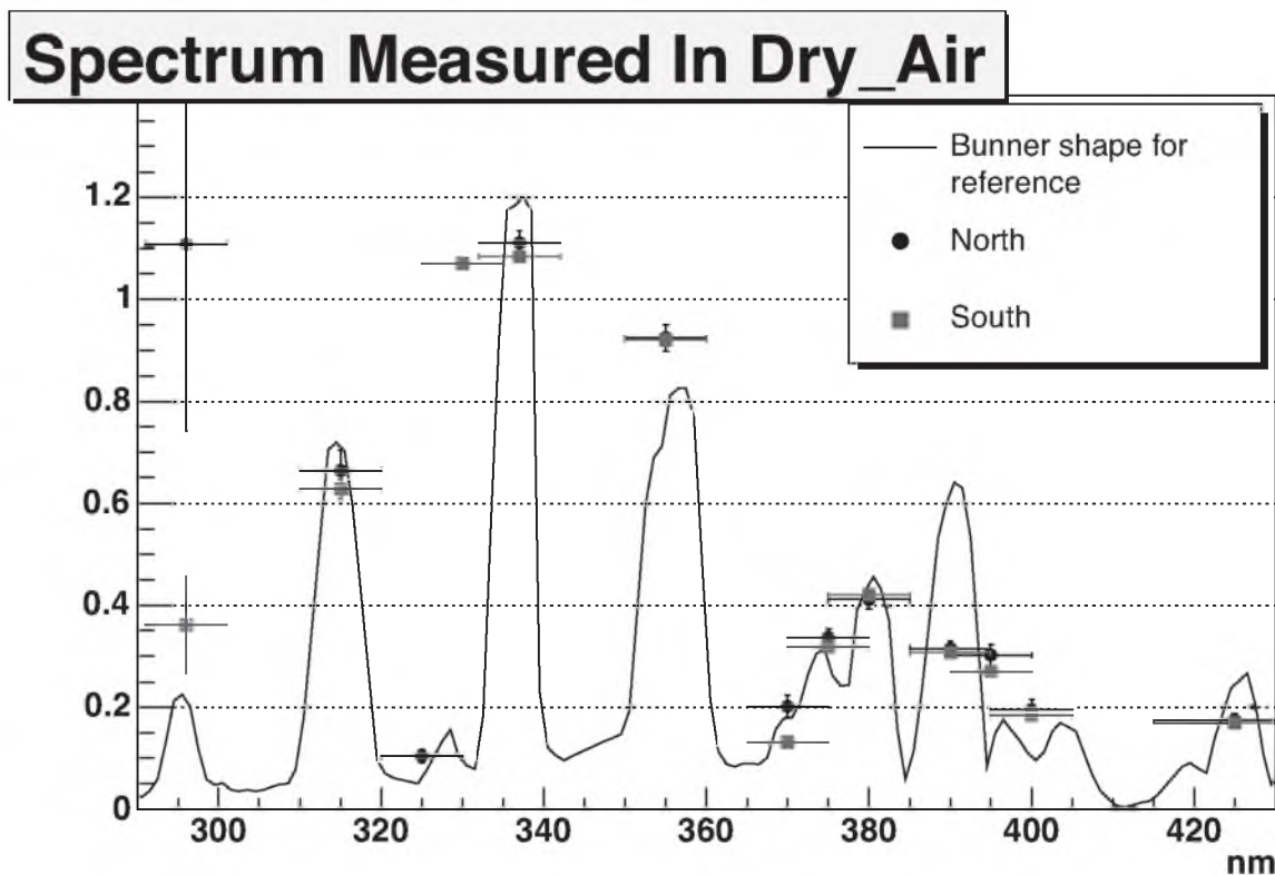
Figure 3.29. The nitrogen fluorescence spectrum as measured by the FLASH collaboration: the spectrum calculated by Bunner is shown as a black line for reference. This measurement done by the FLASH collaboration is used for the analysis in this dissertation.
