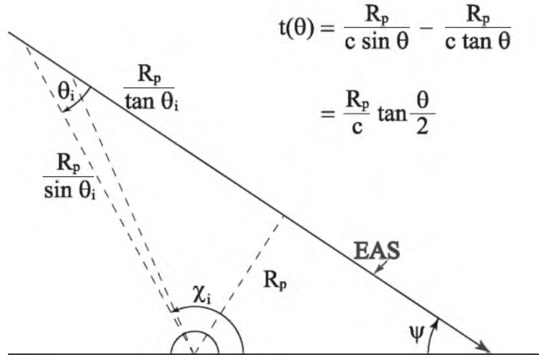
Figure 5.10. Diagram indicating the geometry of the shower within the SDP and parameter names: the diagram shows how the PMT trigger time is related to a given pointing angle within the SDP.
