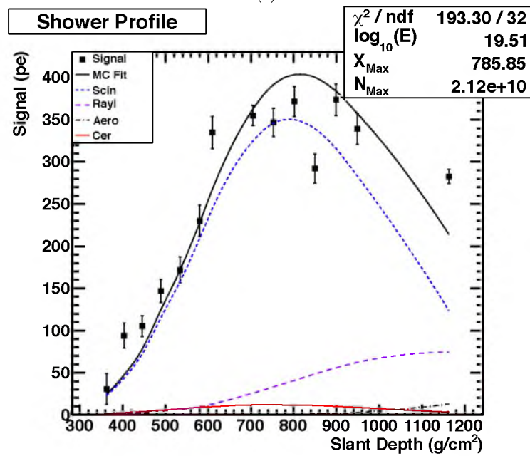
Figure A.5. Continuation of the fourth highest energy event in the Middle Drum hybrid data set: it was recorded on 09/29/2008 at 7:44:10 UTC. Shown are (c) the timing vs. angle plot for the geometry reconstruction, and (d) the plot of the shower profile (signal as a function of atmospheric depth).
