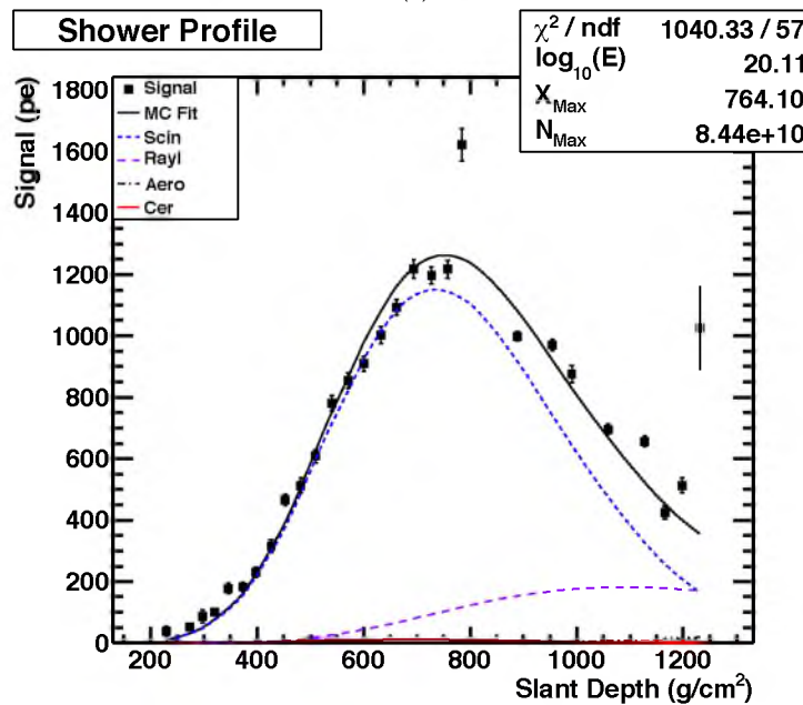
Figure A.2. Continuation of the highest energy event in the Middle Drum hybrid data set: shown are (c) the timing vs. angle plot for the geometry reconstruction, and (d) the plot of the shower profile (signal as a function of atmospheric depth).
