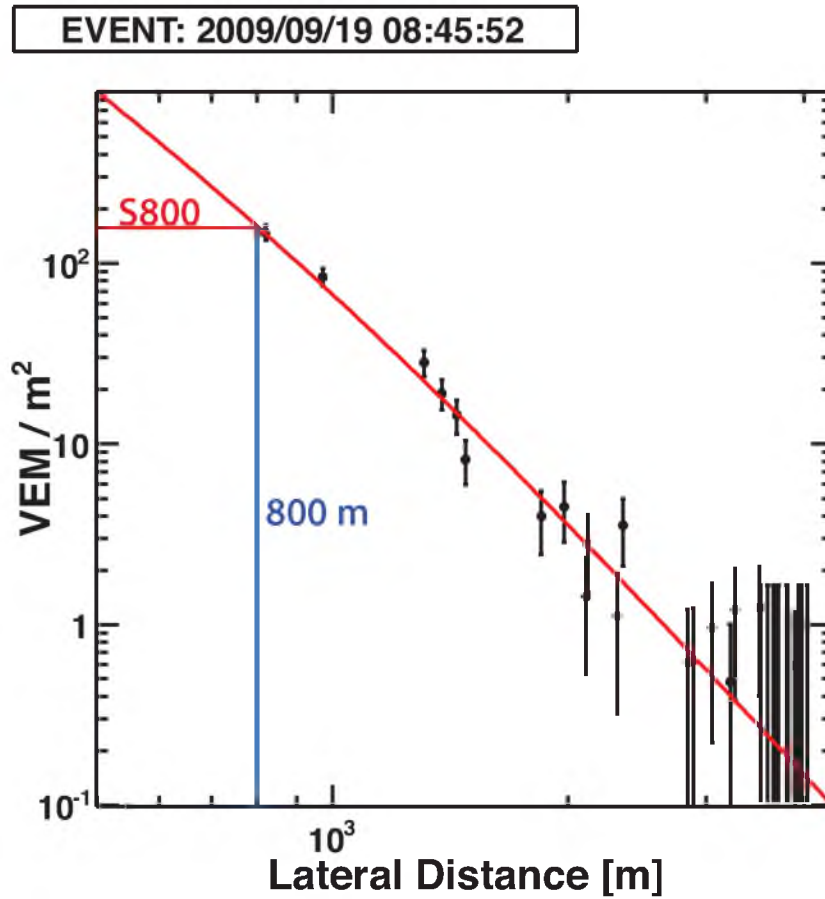
Figure 5.5. The fit to the Lateral Distribution Function (LDF): the pulse height (VEM/m 2 ) is plotted as a function of the lateral distance from the shower axis for event 2009/09/19 08:45:52. The estimated signal size, S800, (from the LDF fit) at a distance of 800 m from the shower core is used to determine the energy of the primary particle.
