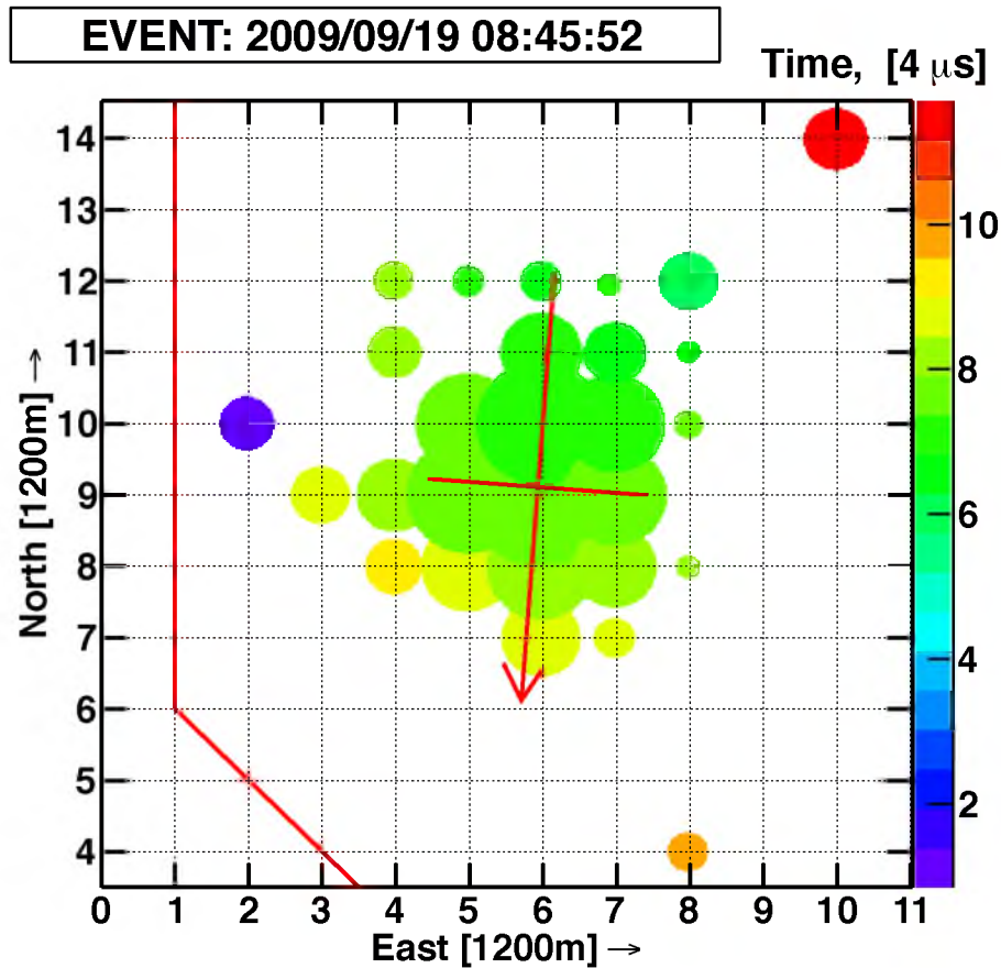
Figure 5.3. SD event display: the Center Of Gravity (COG) core position is shown where the arrow crosses the line for event 2009/09/19 08:45:52. The COG core is calculated using only the pulse heights of the signals from triggered SDs. The direction of the arrow is determined by studying the pulse heights of the elliptical footprint of the shower on the ground and effectively finding the semimajor axis of the ellipse. The COG core position is the starting point for the SD timing fit and lateral distribution fit, and the uncertainty in the COG shower core, \sigma_{\mathbf{R}_{COG}} , is calculated as 170 m. Note that the triggered counters which are not contiguous (e.g., 0210, 0804, and 1014) are removed from the event in the SD Pass1 program.
