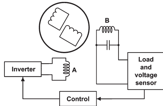
Fig. 1. Inverter-assisted induction generator.
