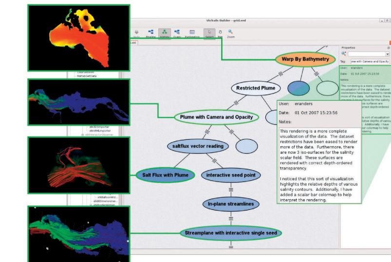
Figure 4. VisTrails. 10 The provenance management system exposes incremental changes to a visualization of model results to users. This provenance history (coupled with explicit annotations as in the inset) lets even nonexperts build new products “by example” instead “from scratch.”
