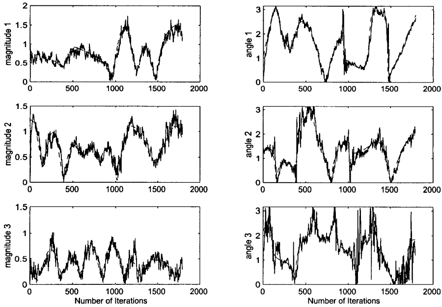
Fig. 2. Evolution of the channel parameters with K = 8 users and f_{d_{max}} = 100 Hz. Dash line: actual parameters. Solid line: estimated parameters. The channel estimation method was described in (12).
