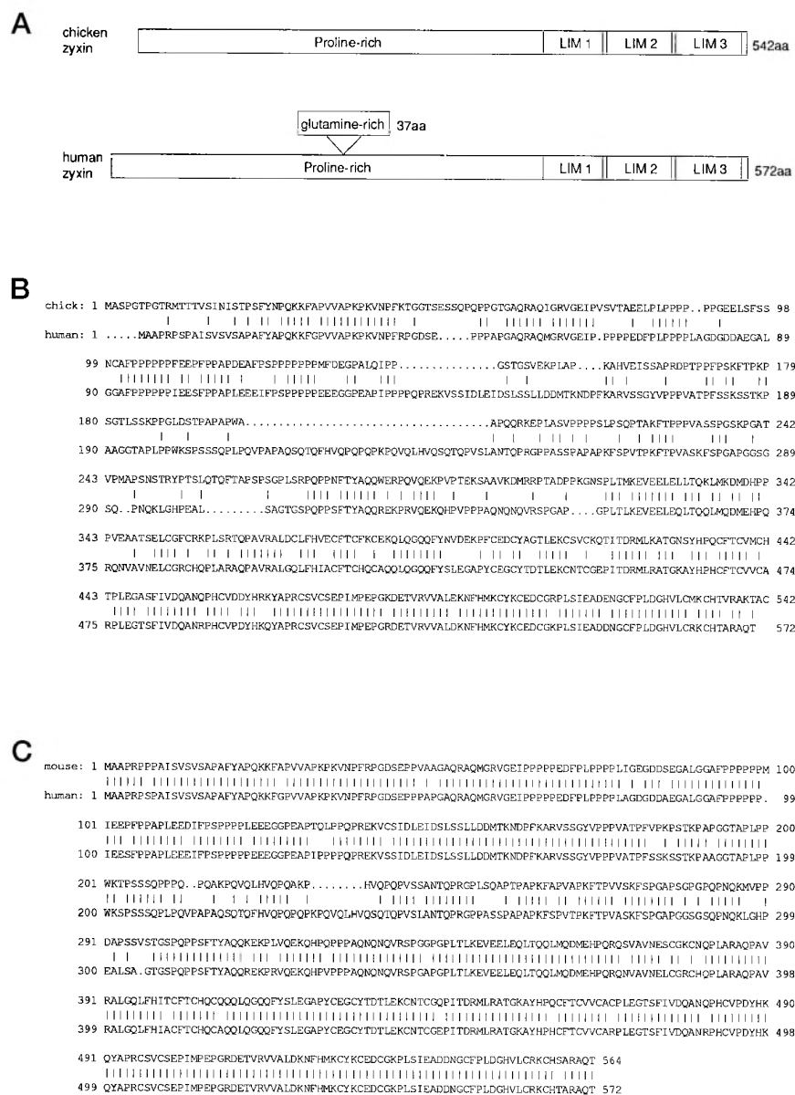
FIG. 2. Comparison of the amino acid sequences of chicken and human zyxin. A , a schematic representation of chicken and human zyxin proteins. The global architecture of the protein is conserved in the human and avian proteins; however, the human protein exhibits a few short sequences that are not found in the avian protein. aa , amino acids. B , a comparison of the amino acid sequences of chicken and human zyxin. The proteins display substantial similarity, particularly in the C-terminal LIM region. Identical residues are indicated by vertical lines. C , a comparison of the amino acid sequences of human and mouse zyxin. Identical residues are indicated by vertical lines.
