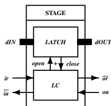
Fig. 1. Stage = Latch and Controller
