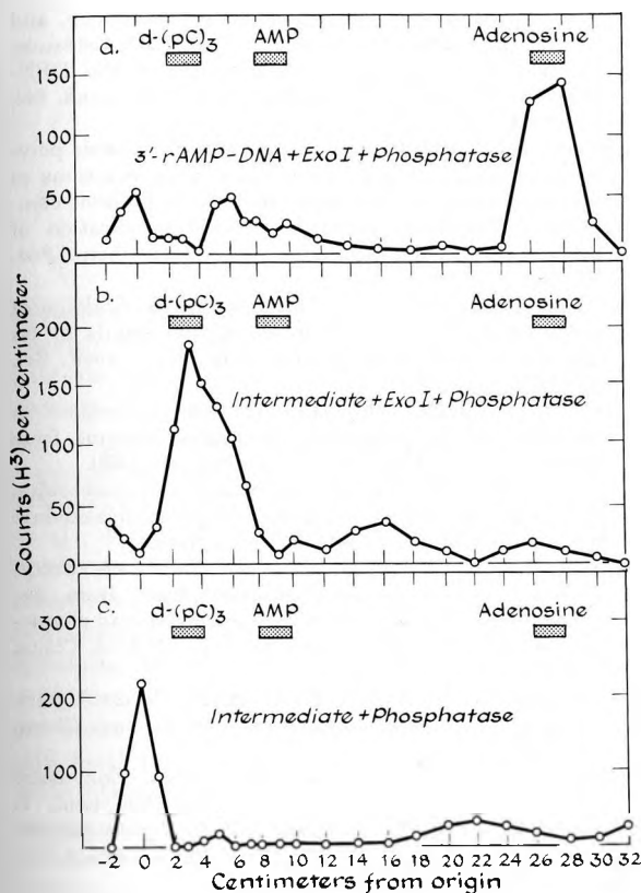
FIGURE 9. Paper electrophoresis of DNA-adenylate intermediate and DNA chains with riboadenylate at their 3' termini ( 3' -rAMP-DNA) after treatment with exonuclease I (Exo I) and phosphatase. Three reaction mixtures (0.2 ml each) were prepared containing 80 mM glycine-NaOH, pH 9.5, 8 mM \text{MgCl}_2 , and 2.5 mM \beta -mercaptoethanol. To one (reaction mixture a) were added single-stranded DNA chains with ^3\text{H} -AMP at their 3' termini (60 \mu\text{g} DNA, 800 count/min), 17 units of exonuclease I (Lehman and Nussbaum, 1964) and 5 units of phosphatase. To the other two were added heat-denatured DNA-adenylate (19 \mu\text{g} DNA, 250 count/min) and either exonuclease I and phosphatase (b) or phosphatase alone (c). The reaction mixtures were incubated at 37^\circ\text{C} for 30 min, then chromatographed for 18 hr in the 1-propanol ammonia-water system (Lehman et al. 1962). The paper was dried, the nucleotides identified, and the radioactivity determined. The values shown correspond to the total number of counts, corrected for background recorded for each strip.
