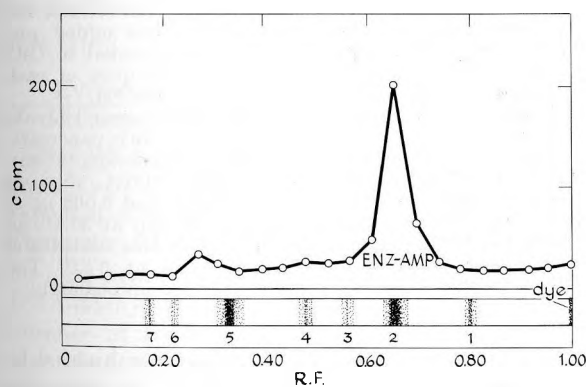
FIGURE 4. Disc gel electrophoresis of enzyme-AMP. A reaction mixture (1.0 ml) containing 0.3 \mu M 32 P-DPN ( 3 \times 10^8 count/min/ \mu mole) labeled in both phosphate groups, 10 mM Tris-HCl, pH 8.6, 3 mM MgCl 2 and 30 units of enzyme was incubated for 10 min at 30°C, then subjected to polyacrylamide gel electrophoresis according to Jovin et al. (1964). After staining with amido black, the gel was cut into 2 mm slices and radioactivity of the slices determined.
