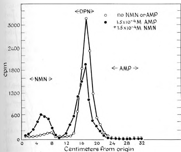
FIGURE 3. Exchange reaction between NMN and DPN. Two reaction mixtures (0.1 ml) were prepared containing 10 mM Tris-HCl, pH 8.0, 2 mM MgCl 2 , 1 mM EDTA, 1.45 \mu M 32 P-DPN ( 2 \times 10^8 count/min/ \mu mole) labeled in both phosphate groups and 0.5 unit of joining enzyme; one reaction mixture was made 0.15 mM in AMP and 0.15 mM in NMN. Both reactions were incubated at 30°C for 20 min; an additional 1.8 units of enzyme were added to each and the mixtures were incubated again for 40 min at 30°C. The reaction mixtures were heated at 100° for 2 min, then subjected to paper electrophoresis (5000 volts for 60 min) in 0.015 M citrate buffer, pH 5.5, with AMP, DPN and NMN as markers. The paper was cut into strips (1 \times 4 cm) and their radioactivity determined. The small peak of radioactivity migrating slightly ahead of NMN in the control mixture is an impurity in the 32 P-DPN preparation.
