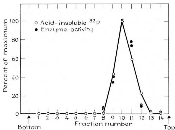
FIGURE 5. Demonstration of enzyme-AMP by sucrose density gradient sedimentation. The reaction mixture (2.0 ml) contained 10 mM Tris-HCl, pH 8.0, 7 mM MgCl 2 , 1 mM EDTA, 50 \mu g/ml of bovine plasma albumin, 0.5 \mu M 32 H-DPN ( 1.8 \times 10^8 count/min/ \mu mole), and 20 units of joining enzyme. After incubation for 30 min at 30°C, 40 \mu moles of EDTA, pH 8.7, and 0.2 mg of bovine plasma albumin were added, and the mixture dialyzed against 1 liter of 0.5 M (NH 4 ) 2 SO 4 , 10 mM Tris-HCl, pH 8.0 (3 changes). The dialyzed solution which contained 1400 count/min/ml was centrifuged in a 5–20% sucrose gradient containing 0.5 M (NH 4 ) 2 SO 4 , 10 mM Tris-HCl, pH 8.0 and 0.1 mg/ml albumin, at 38,000 rpm for 26 hr at 10°. At the end of the run, 20-drop fractions were collected; 0.1 ml-aliqouts of each fraction were heated at 100°C for 2 min and acid-precipitable 32 P was determined. The remainder of each fraction was used to assay joining enzyme activity (Olivera and Lehman, 1967a).
