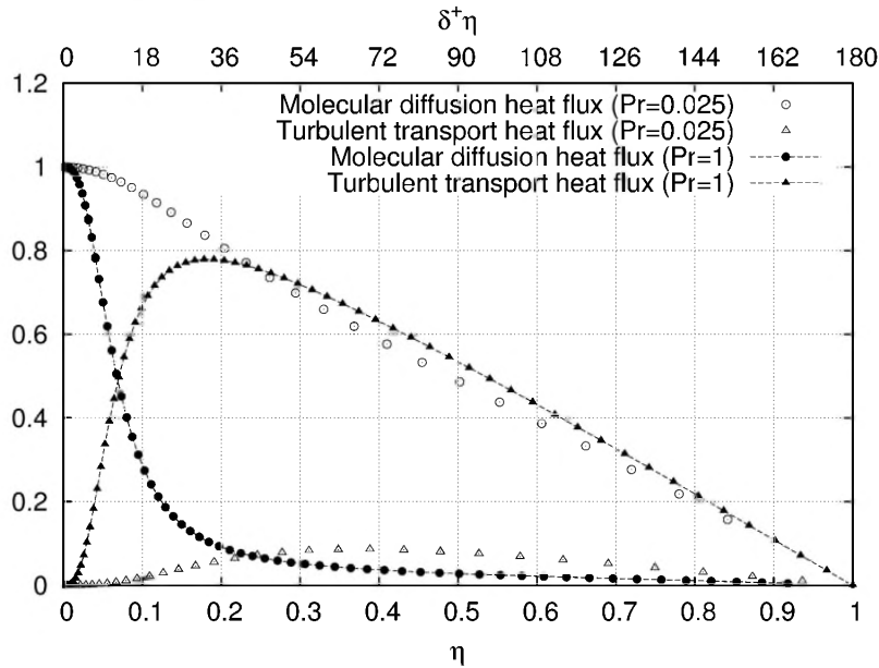
Figure 2: The molecular diffusion heat flux \frac{d\Phi}{d\eta} and turbulent heat flux, T = \langle v^+ \frac{\theta}{\theta_\tau} \rangle for two Prandtl numbers, in one case Pr \ll O(1) and in the other, Pr = 1 . Note that for Pr \ll 1 and not too high Reynolds number (i.e., Re_\tau = 180 ), \frac{d\Phi}{d\eta} is always larger than T .
