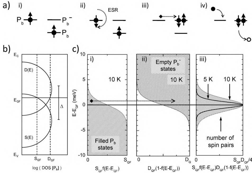
FIG. 4. (a) Cartoon of spin-dependent tunneling between two adjacent uncharged P_b centers where the ground-state energy of one P_b matches the P_b^-/P_b charging energy of the other. (i) Initially, the pair is in a triplet state and tunneling is not possible. (ii) Once the spin of one P_b state is changed the pair has singlet content and tunneling (iii) is allowed. (iv) An excess charge-carrier pair recombines as it discharges the two charged P_b states. (b) Sketch of DOS of P_b centers within the c -Si band gap (Ref. 5). Note that DOS's of P_b and P_b^- are assumed to be identical but shifted by the correlation energy \Delta . (c) Plot for T=10 K of the number of (i) filled P_b states, (ii) filled P_b^- states, and (iii) tunneling pairs as a function of energy about the quasi-Fermi level E_{QF} . The sharper pair distribution for T=5 K is indicated by the solid line. The plot illustrates that there are fewer pairs of adjacent P_b and P_b^- with matching energies when T decreases.
