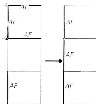
FIG. 1. Random, or “ordered but geometrically frustrated?” Heavy lines are AF bonds, light lines are ferromagnetic. The apparently disordered ladder on the left turns into an ordered (but equally frustrated!) ladder after two spins are “flipped” by a gauge transformation: S_1 \rightarrow -S_1 and S_2 \rightarrow -S_2 .
