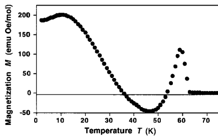
Figure 8. Temperature-dependencies of the magnetization for Mn^{II}_{1.80}Fe^{II}_{0.54}Ni^{II}_{0.66}[Cr^{III}(CN)_6]_2 \cdot 15.2H_2O , revealing compensation temperatures at 35 K and 53 K.
