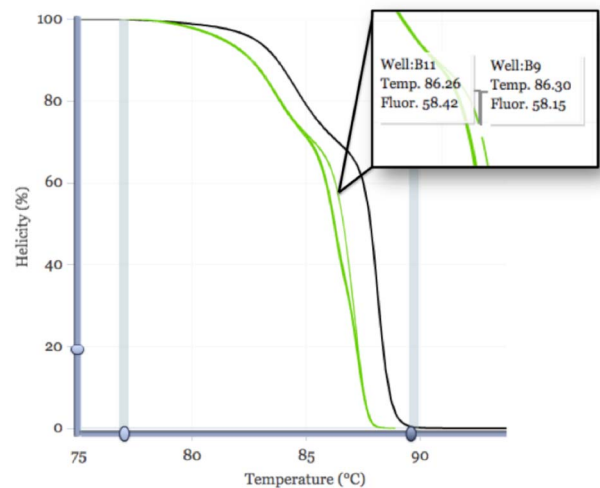
Fig. 4. uAnalyze melting curve analysis identifies heterozygous c. 1090G > A in exon 9 (amplicon 9b) of CYBB after experimental curve overlay. Experimental data (green curves) are normalized after exponential background subtraction and overlaid between 5 and 15 percent helicity. Hovering over the abnormal curves pops up a box that reveals the physical sample locations, along with the temperature and fluorescence of the cursor. The black curve is predicted by thermodynamics and shows the two domains also observed in the experimental curves.
