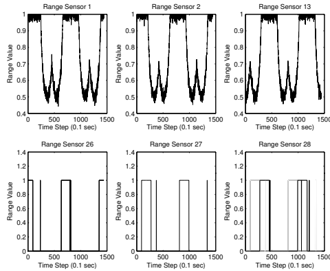
Figure 2: Sensor data showing translation symmetry: Row 1 shows sensors 1, 2, and 13; Row 2 shows compass sensors 27,28, and 29.
