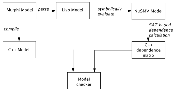
Fig. 3. Murphi verification flow with partial order reduction
