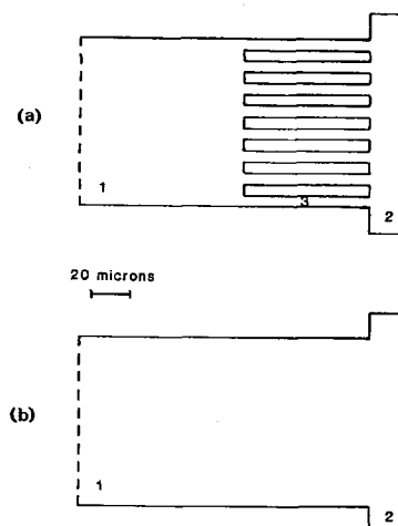
Fig. 1. Electrode masks for long junctions (a) with fingers (b) no fingers. Electrode 1, Junction area 2, Equally spaced fingers 3.
