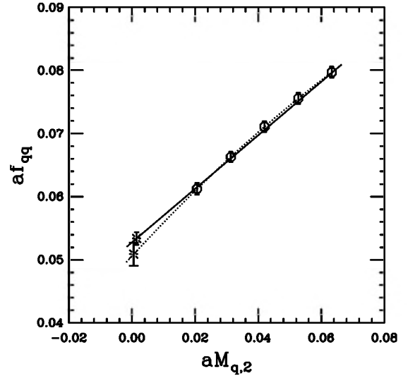
FIG. 6. The light-light pseudoscalar decay constant, f_{qq} , vs a\bar{M}_{q,2} for set J . The solid line is a linear fit; the dotted line, the alternative quadratic fit. The fits have \chi^2_{\text{cut}}/\text{d.o.f.} = 1.1 and 0.005 , respectively, with \lambda_{\text{cut}} = 1 (1 eigenvector of 5 kept). The bursts are the extrapolated points where \bar{M}_{q,2} takes its physical value (i.e., \kappa = \kappa_{u,d} ). The burst on the dotted line has been displaced slightly for clarity.
