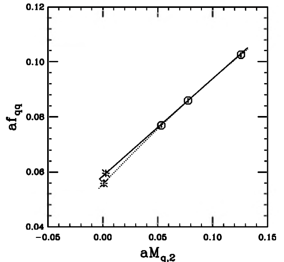
FIG. 7. Same as Fig. 6, but for set R. The linear fit (solid line) has \chi^2_{\text{cut}}/\text{d.o.f.} = 8.7 , \lambda_{\text{cut}} = 1 (1 eigenvector of 3 kept); while the quadratic fit (dotted line) has no degrees of freedom.
