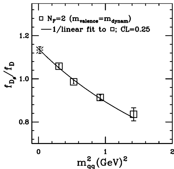
FIG. 30. Chiral extrapolation of f_{D_s}/f_D at \beta=5.5 (sets P, M, O, N) with the light valence quark mass in f_D equal to the dynamical quark mass. The quantity 1/(f_{D_s}/f_D) is fit to a linear function.
