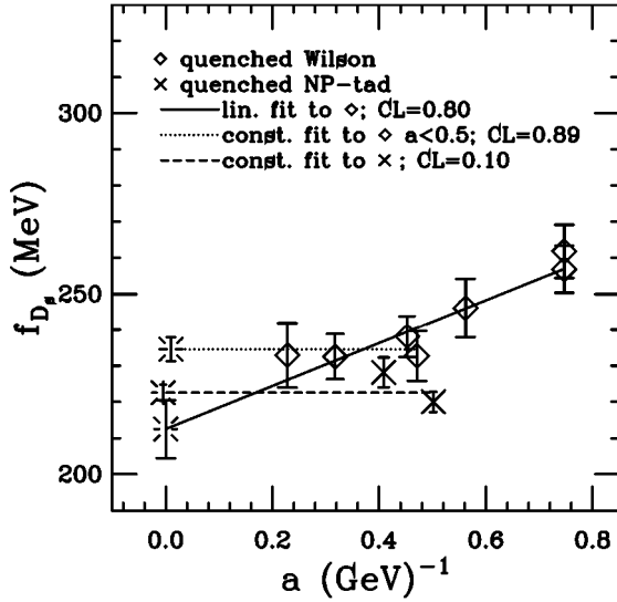
FIG. 21. f_{D_s} vs a for quenched lattices. Labels are the same as in Fig. 18, but the NP-IOY points have been omitted because the perturbative calculation is not available at the relevant lattice masses.
