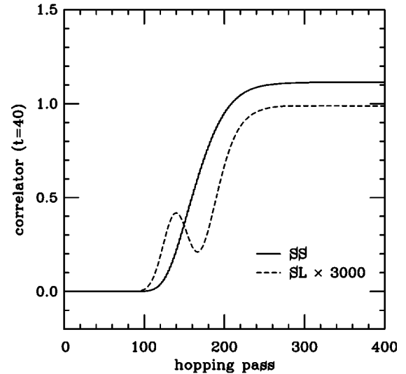
FIG. 1. Convergence of the hopping parameter expansion for heavy-light pseudoscalar meson correlators on set D. \kappa_Q=0.1456 , while \kappa_q=0.1507 , the lightest of the three light quarks analyzed on this set. The values of the smeared-smeared and smeared-local correlators at t=40 (half-way across the lattice) are shown with the solid and dashed lines, respectively.
