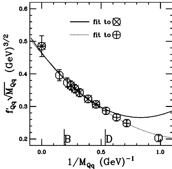
FIG. 15. f'_{Qq} \sqrt{M_{Qq}} vs 1/M_{Qq} for set CP (quenched Wilson). The scale is set by f_\pi . The solid line is fit (1) (“heavier-heavies”) and includes points marked with a cross. The dotted line is fit (2) (“lighter-heavies”) and includes points marked with a plus. The fits have \chi^2_{\text{cut}}/\text{d.o.f.}=0.4 and 0.9 , respectively, with \lambda_{\text{cut}}=1 (1 eigenvector kept).
