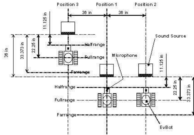
Figure 8: Experimental Setup.
