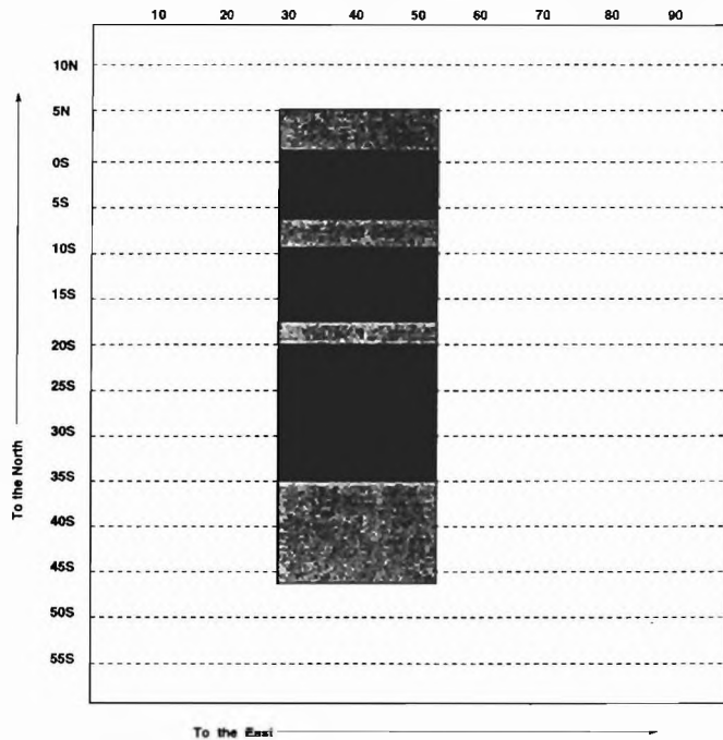
Fig. 3. The schematic plan of the RWMC Cold Test Pit. 1 - nonconductive zones (Earth berm); 2 - conductive zones (random dump drums and boxes); 3 - conductive zone (stacked drums, contains 700 drums).
