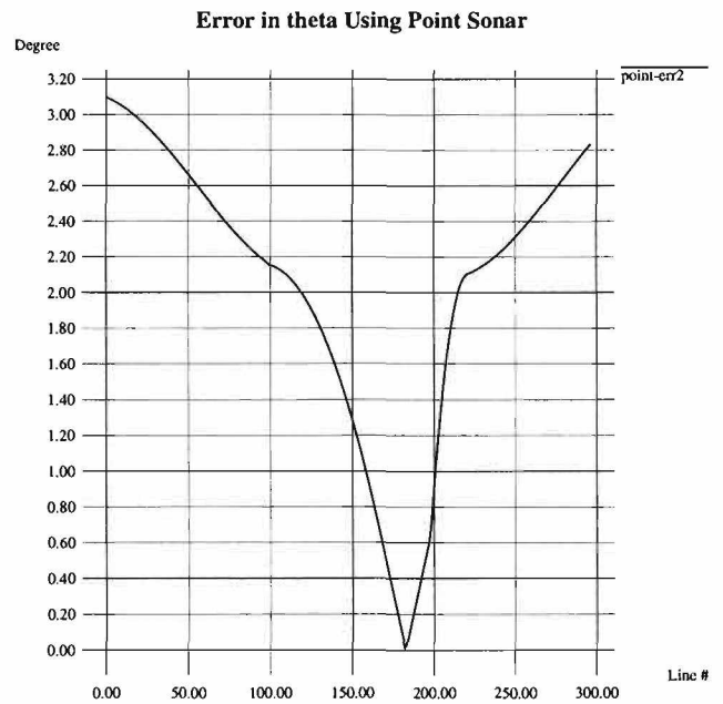
Figure 14: The error in both cases using synthetic data.
