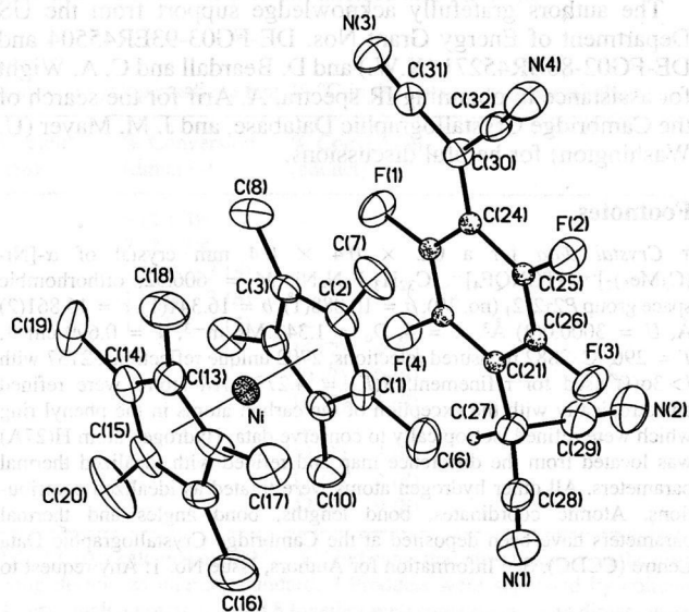
Fig. 1 ORTEP drawing depicting the atom labelling of [Ni(C 5 Me 5 ) 2 ] + [HTCNQF 4 ] - ; atoms shown as 30% probability ellipsoids
