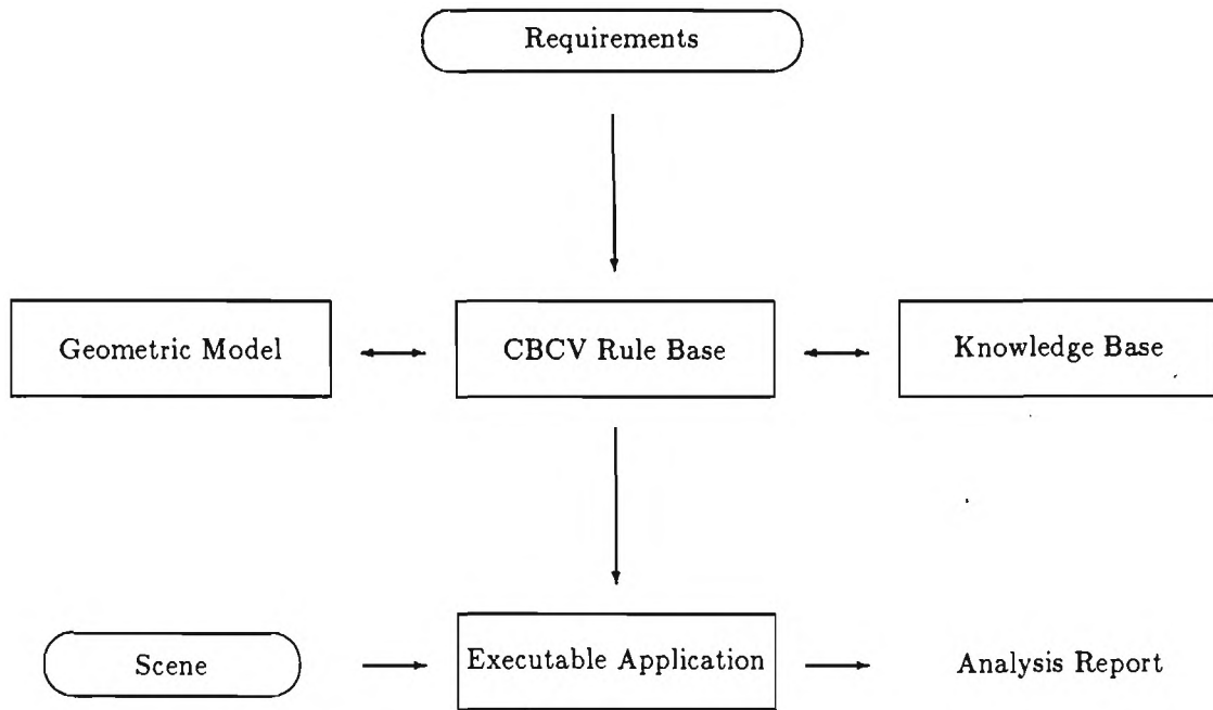
Figure 11: Vision Paradigm
