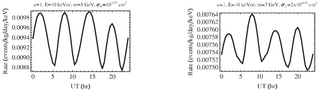
FIG. 7. Signal rate as a function of UT during 24 hours for a solid Ne detector operating at T = 23 K at Gran Sasso for E = 10 keVee, Q = 0.25 , c = 1 , \sigma_v = 300 km/s, V_{\text{lab}} = 228.4 km/s and for (a) m = 5 GeV and \sigma_p = 10^{-39} cm ^2 , and (b) m = 7 GeV and \sigma_p = 2 \times 10^{-40} cm ^2 .
