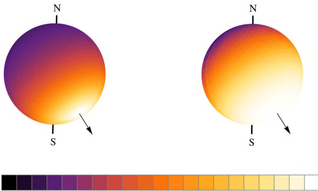
FIG. 3 (color online). (a) f_{\text{WIMP}}(\hat{\mathbf{v}}, v_q) [in Eq. (13)] rescaled to be between 0 and 1 plotted on the sphere of velocity directions \hat{\mathbf{v}} and (b) \hat{f}_{\text{lab}} [rescaled as in Eq. (15)] plotted on the sphere of recoil directions using the HEALPix for I recoils with E_R = 10 keV, m = 30 GeV (thus v_q = 304.6 km/s). V_{\text{lab}} = 288.3 km/s, and \sigma_v = 300 km/s. The arrow shows the direction of the average velocity of the WIMP wind, -\mathbf{V}_{\text{lab}} . The North and South celestial poles are also indicated. The color scale/gray scale shown in the horizontal bar corresponds to values between 0 (black) and 1 (white) in intervals of 0.05.
