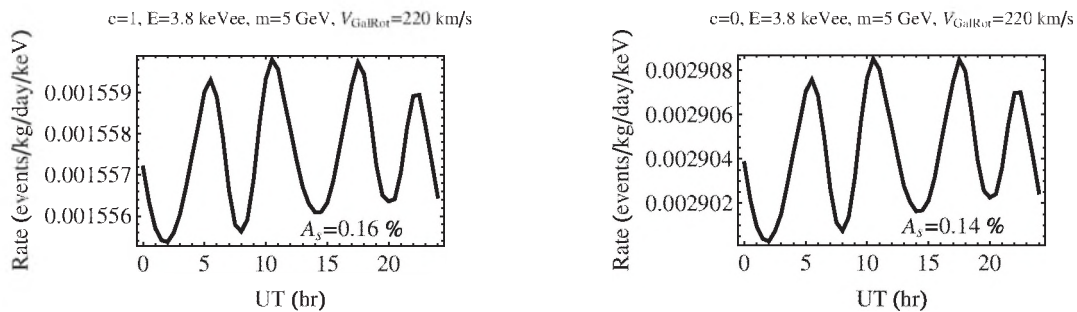
FIG. 6. Signal rate as function of UT during 24 hours for E = 3.8 keVee and m = 5 GeV, with V_{\text{lab}} = 228.4 km/s, \sigma_v = 300 km/s, \sigma_p = 2 \times 10^{-40} cm 2 , and Q_{\text{Na}} = 0.2 , Q_{\text{I}} = 0.09 for (a) c = 1 and (b) c = 0 . The daily modulation is not observable in both cases.
