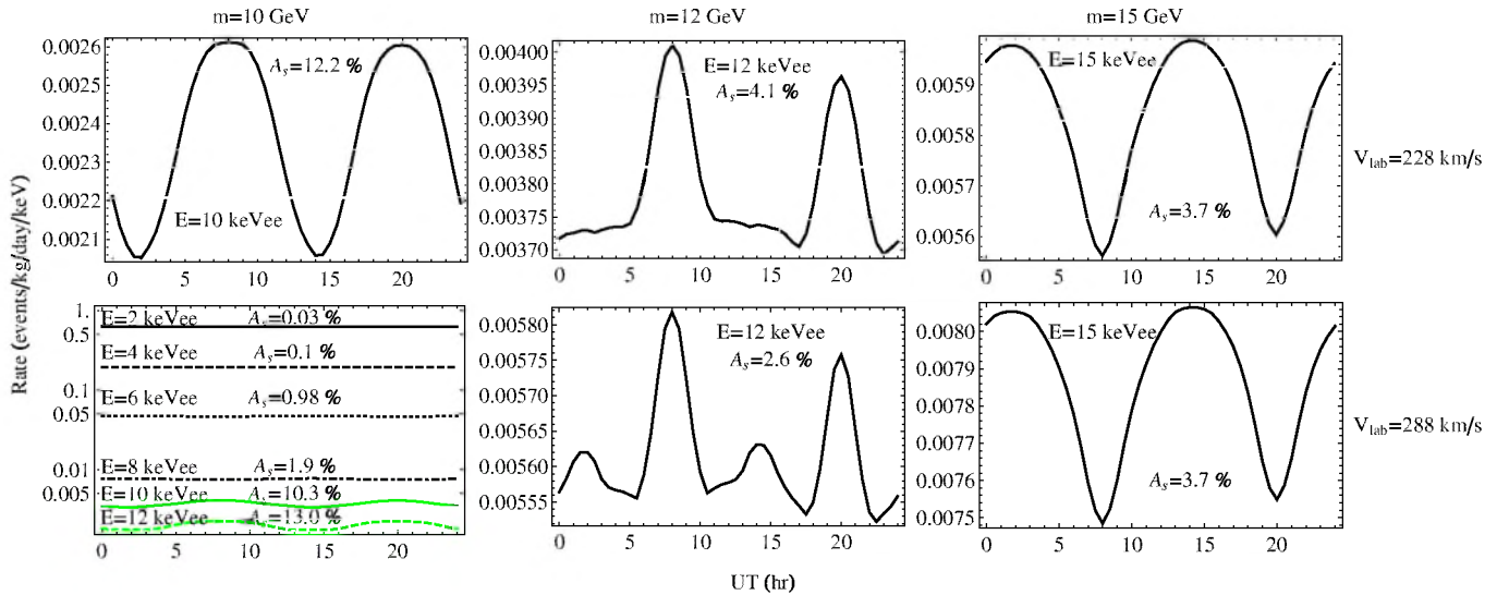
FIG. 5 (color online). Signal rate (in events/kg-day/keVee) as a function of the universal time (UT) during 24 hours for m = 10 GeV, 12 GeV, and 15 GeV for different energies. The parameters used are \sigma_v = 300 km/s, Q_{\text{Na}} = 0.2 , Q_{\text{I}} = 0.09 , \sigma_p = 2 \times 10^{-40} cm 2 , c = 1 for temperature effects, a crystal temperature of T = 293 K and V_{\text{lab}} = 228.4 km/s (top row) or 288.3 km/s (bottom row).
