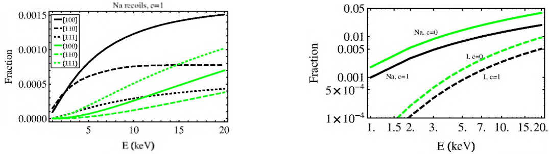
FIG. 1 (color online). Upper bounds to the (a) channeling fractions for single channels \chi_i(E, \hat{\mathbf{q}}) of Na recoils for axial (black lines) and planar (green/gray lines) channels with c = 1 , and (b) geometric channeling fraction P_{\text{geometric}}(E) of Na (solid lines) and I recoils (dashed lines) as a function of the recoil energy E for T = 293 K in with c = 0 (green/gray) and c = 1 (black), always without including dechanneling.
