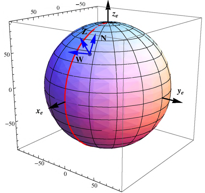
FIG. 8 (color online). Earth’s sphere in the equatorial frame ( \hat{\mathbf{x}}_e, \hat{\mathbf{y}}_e, \hat{\mathbf{z}}_e ) specified with black arrows. The laboratory frame ( \hat{\mathcal{N}}, \hat{\mathcal{W}}, \hat{\mathcal{Z}} ) specified with blue/dark gray arrows is also shown.
