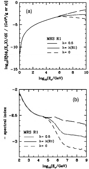
FIG. 7. (a) NLO charm production function E_c^3 d\phi_c(E_c, X)/dX (PDF MRS R1); (b) its spectral index -\partial \ln[d\phi_c(E_c, X)/dX]/\partial \ln E_c . These results are for a height h = 20 km, corresponding to a vertical depth X = 57.12 g/cm 2 (similar results are obtained for other heights).
