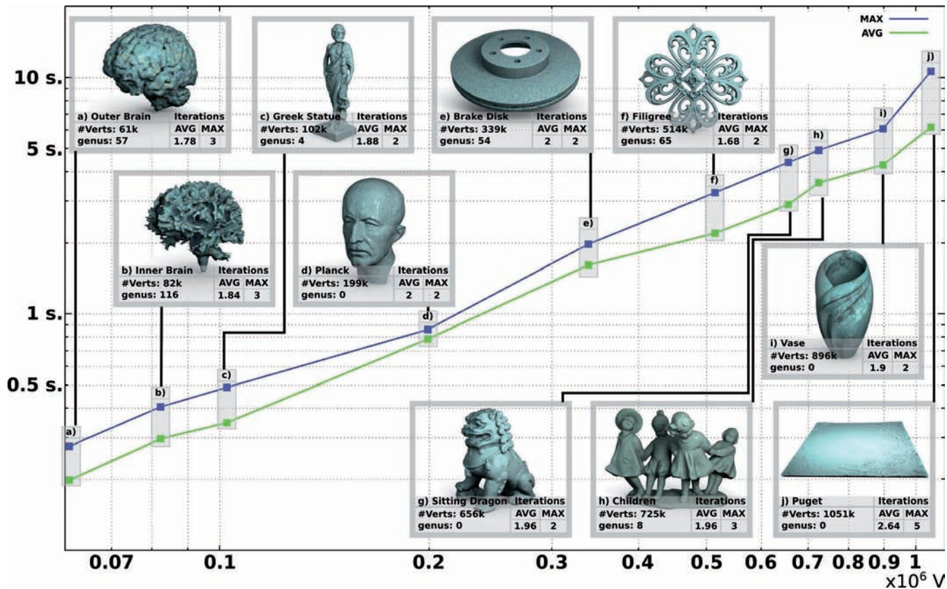
Fig. 8. Running times (log scale) for the simplification of random functions, with a random constraint selection ( C_g^0, C_g^2 ), 50 runs per data-set.
